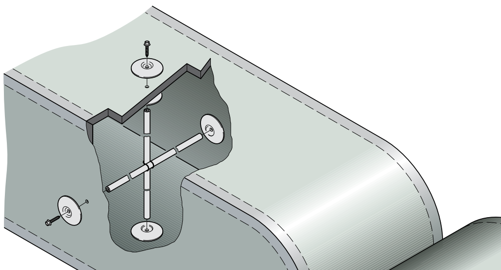
code 21RF01ABT - Antimicrobial aluminium shaped disk
